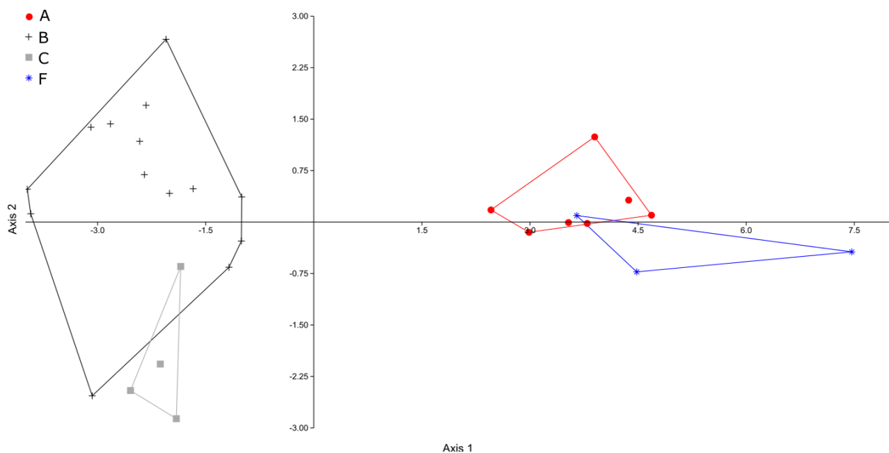
FIGURE 12. Graphical representation of scores for the first two DFA factors separating Megascops atricapilla - M. watsonii clades A, B, C, and F based on measurements of nine shortsong characters (pace, note length, peak frequency, max power, change in note length, change in interval length, change in peak frequency, change in max power, and change in pace).
