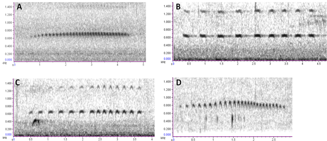
FIGURE 11. Audiospectrograms of shortsongs of Megascops atricapilla - M. watsonii clades A, B, C, and F. (A) Clade A: Venezuela, Rio Grande (Paul Schwartz, ML 59359); (B) Clade B: Brazil, Mato Grosso (Curtis Marantz, ML 126830); (C) Clade C: Brazil, Serra dos Carajás (Curtis Marantz, ML 126657); and (D) Clade F: Brazil, Parque Estadual Intervales, São Paulo (Dan Lane, XC 75524).
