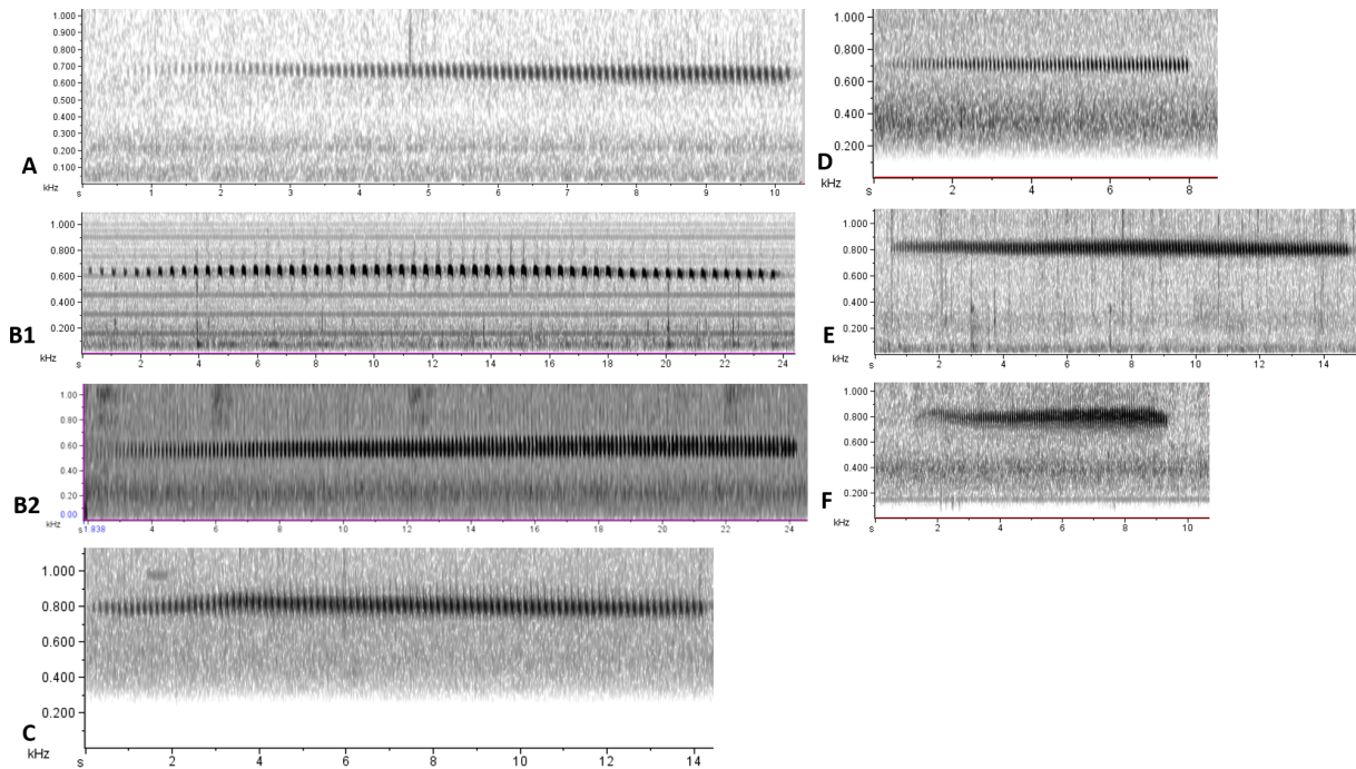
FIGURE 8. Examples of longsong audio spectrograms from clades A–F of the Megascops atricapilla - M. watsonii complex. (A) Clade A: Venezuela, Rio Cuyuni (Paul Schwartz, ML 59376); (B1) Clade B: Peru, Madre de Dios (Ted Parker III, ML 11496 = locality B26 in Fig. 1); (B2) Clade B: Venezuela, Rio Cassiquiare (Paul Schwartz, ML 59397 = locality B23 in Fig. 1); (C) Clade C: Brazil, Serra dos Carajás (Sidnei Dantas, XC 22514); (D) Clade D: Brazil, IPEAN, Belém (Paul Schwartz, ML 59395); (E) Clade E: Brazil, Usina Serra Grande, Ibateguara, Alagoas (Curtis Marantz, ML 127980); (F) Clade F: Brazil, Caetetus Ecological Station, São Paulo (Alexandre Aleixo, ML 94909). Each sonogram is typical of a given clade, except for Clade B, where a slow-paced song (less than 4 notes/s), and a fast-paced song (more than 6 notes/s) are shown. The slow-paced individuals are all from the south bank of the Amazon River, while most of the fast-paced Clade B specimens come from north of the Amazon, except for some samples from the lower Inambari and Rondonia areas of endemism in Brazil (see Fig. 9).
