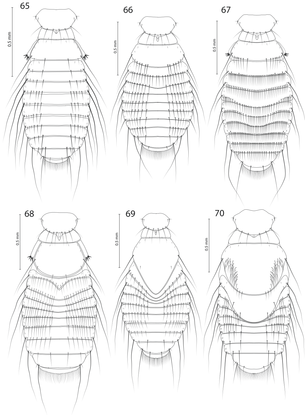
Figs. 65–70. Dorsal view of thorax and abdomen of females: 65, M. pycnonoti ; 66, M. leucophthalmi ; 67, M. poliogasteri ; 68, M. scleruri ; 69, Myrsidea sp. from Erythrura trichroa ; 70, M. chapensis .
