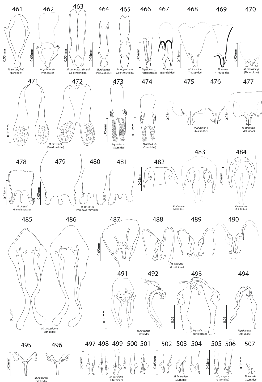
Figs. 461–507. Male genital sac sclerites. 461, M. eurocephali . 462, M. prionopsis . 463, M. ananthakrishnani . 464, Myrsidea sp. from Pardalotus quadragintus . 465, M. argenteauris . 466, Myrsidea sp. from Pardalotus punctatus . 467, M. zenae . 468, M. flaveolae . 469, M. spizae . 470, M. mitrospingi . 471 and 472, M. crassipes . 473, Myrsidea sp. from Gracula religiosa palawanensis . 474, Myrsidea sp. from Gracula religiosa . 475 and 476, M. pectinata . 477, M. strangeri . 478, M. piageti . 479–481, M. suthorae . 482 and 483, M. srivastava . 484, M. amandava . 485 and 486, M. cyrtostigma . 487–490, M. estrildae . 491 and 492, Myrsidea sp. from Estrilda nonnula . 493, Myrsidea sp. from Padra oryzivora . 494, Myrsidea sp. from Lonchura castaneothorax . 495–496, Myrsidea sp. from Taeniopygia guttata . 497–501, M. cucullaris (500 and 501 formerly as M. lyali ). 502–504, M. lengerkeni . 505 and 506, M. pungens . 507, M. teraokai . Except for figures redrawn from other publications, all figures are drawn to the same scale. Scale is shown for redrawn figures if it was present in the original publications. The following figures were redrawn from the following publication: Fig. 463 from Rai (1978); Fig. 465 from Price et al. (2006); Figs. 467 and 469 from Price and Dalgleish (2006); Fig. 473 from Eduardo and Villa (2011); Fig. 479 from Lei et al. (2020); Fig. 499 from Fedorenko (1983); Fig. 500 from Klockenhoff (1984).
