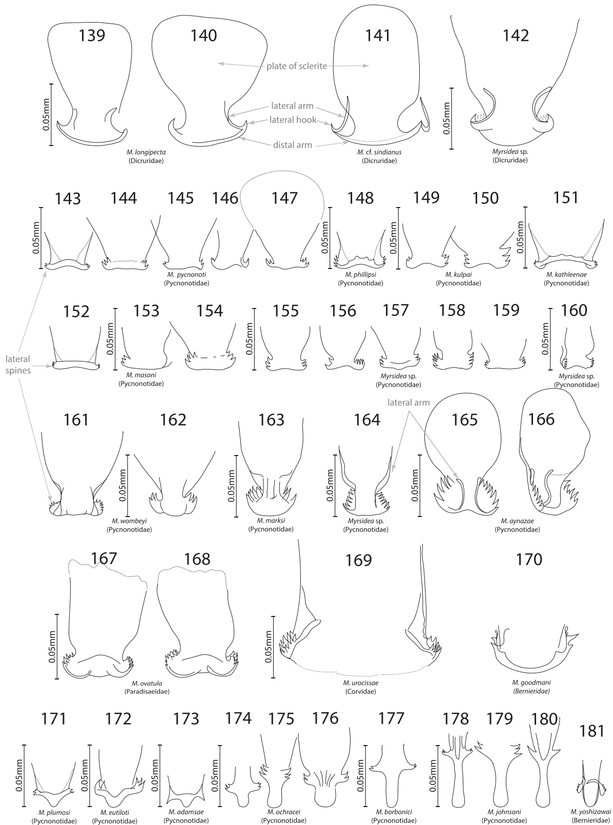
Figs. 139–181. Male genital sac sclerites. 139–140, M. longipecta . 141, M. cf. sindianus (from Dicurus paradiseus ). 142, Myrsidea sp. from Dicurus bracteatus . 143–147, M. pycnonoti . 148, M. philipsi . 149 and 150, M. kulpai . 151, M. kathleenae . 152–154, M. masoni . 155–159, Myrsidea sp. from Bleda notatus . 160, Myrsidea sp. from Arizelocichla tephrolaema . 161 and 162, M. wombeyi . 163, M. marksi . 164, Myrsidea sp. from Eurillas latirostris . 165 and 166, M. aynazae . 167 and 168, M. ovatula . 169, M. urocissae . 170, M. goodmani . 171, M. plumosi . 172, M. eutiloti . 173, M. adamsae . 174–176, M. ochracei . 177, M. borbonici . 178–180, M. johnsoni . 181, M. yoshizawai . Except for figures redrawn from other papers, all figures are drawn to the same scale. Scale is shown for redrawn figures if it was present in the original papers. The following figures were redrawn from the following publications: Figs. 143, 148, 151, 171, 173, 174, 177, and 178 from Hellenthal and Price (2003); Figs. 152 and 161 Johnson and Price (2006); Figs. 170 and 181 from Price and Johnson (2006a).
