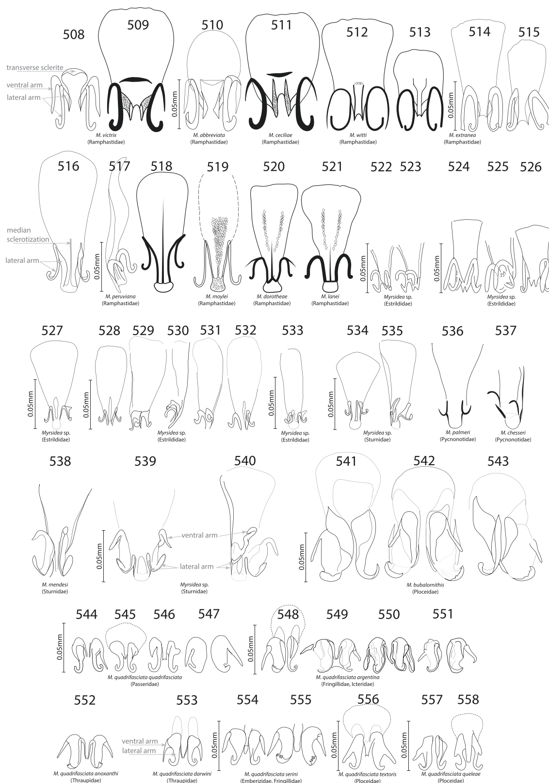
Figs. 508–558. Male genital sac sclerites. 508 and 509, M. vixtrix . 510, M. abbreviata . 511, M. ceciliae . 512, M. witti . 513–515, M. extranea . 516–518, M. peruviana . 519, M. moylei . 520, M. dorotheae . 521, M. lanei . 522 and 523, Myrsidea sp. from Erythrura prasina . 524–526, Myrsidea sp. from Erythrura trichroa . 527, Myrsidea sp. from Cryptospiza salvadorii . 528–532, Myrsidea sp. from Cryptospiza reichenovii . 533, Myrsidea sp. from Nigrita canicapillus . 534, Myrsidea sp. from Notopholia corusca . 535, Myrsidea sp. from Lamprolornis ornatus . 536, M. palmeri . 537, M. chesleri . 538, M. mendesi . 539, Myrsidea sp. from Lamprolornis purpuroptera aenocephalus . 540, Myrsidea sp. from Lamprolornis caudatus . 541, M. bubalornithis . 544–547, M. quadrifasciata quadrifasciata (Passeridae). 548–551, M. q. argentina (Fringillidae, Icteridae). 552, M. q. anoxanthi (Thraupidae). 553, M. q. darwini (Thraupidae). 554 and 555, M. q. serini (Emberizidae, Fringillidae). 556, M. q. textoris (Ploceidae). 557 and 558, M. q. queleae (Ploceidae). Except for figures redrawn from other publications, all figures are drawn to the same scale. Scale is shown for redrawn figures if it was present in the original publications. The following figures were redrawn from the following publication: Fig. 508 from Waterston (1915); Figs. 509, 511–513, 518, 520, and 521 from Price et al. (2004); Fig. 519 from Hellenthal et al. (2005); Figs. 536–537 from Johnson and Price (2006); Fig. 538 from Tendeiro (1993); Figs. 549–551 from Cicchino and Valim (2015); Fig. 552 from Price and Dalgleish (2007); Fig. 553 from Palma and Price (2010); Figs. 554 and 555 from Klöckenhoff (1984c).
