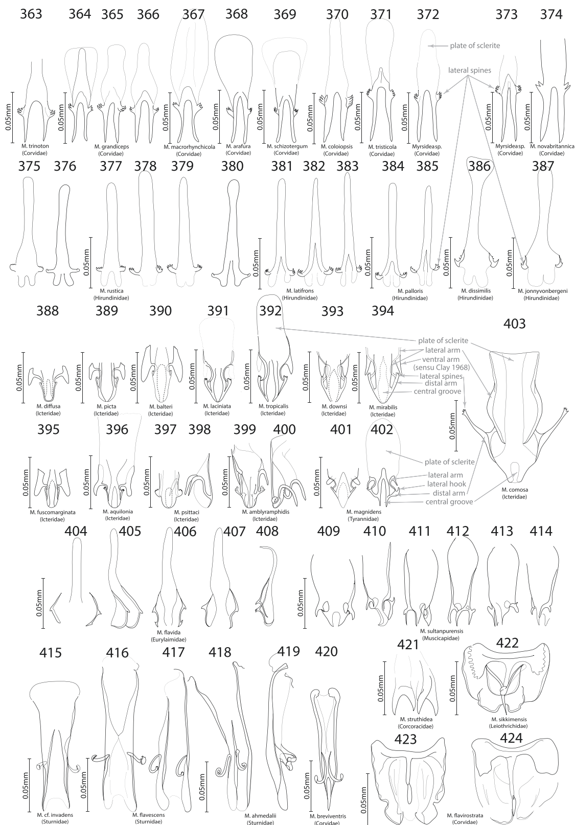
Figs. 363–424. 363, M. triniton . 364–366, M. grandiceps . 367, M. macrorhynchicola . 368, M. arafura . 369, M. schizotergum . 370, M. colioipsis . 371, M. tristicola . 372, Myrsidea sp. from Corvus typicus . 373, Myrsidea sp. from Corvus woodfordi . 374, M. novabritannica . 375–379, M. rustica . 380–383, M. latifrons . 384 and 385, M. palloris . 386, M. dissimilis . 387, M. jonnyvonbergi . 388, M. diffusa . 389, M. picta . 390, M. balteri . 391, M. laciniata . 392, M. tropicalis . 393, M. downsi . 394, M. mirabilis . 395, M. fuscomarginata . 396, M. aquilonia . 397 and 398, M. psittaci . 399 and 400, M. amblyramphidis . 401 and 402, M. magnidens (Fig. 401 as approximate reconstruction). 403, M. comosa . 404–408, M. flvida . 408–414, M. sultanpurensis . 415, M. cf. invadens . 416–417, M. flavesens . 418 and 419, M. ahmedalii . 420, M. vreviventris . 421, M. struthidea . 422, M. sikkimensis . 423 and 424, M. flavirostrata . Except for figures redrawn from other publications, all figures are drawn to the same scale. Scale is shown for redrawn figures if it was present in the original publications. The following figures were redrawn from the following publication: Fig. 374 from Klockenhoff (1980a); Fig. 375 from Conci (1942c); Figs. 376 and 380 from Clay (1949b). Figs. 388–390, 393–395, 397, 398, 401, and 403 from Clay (1968); Figs. 399 and 400 from Valim and Cicchino (2015a); Fig. 402 from Price et al. (2005).
