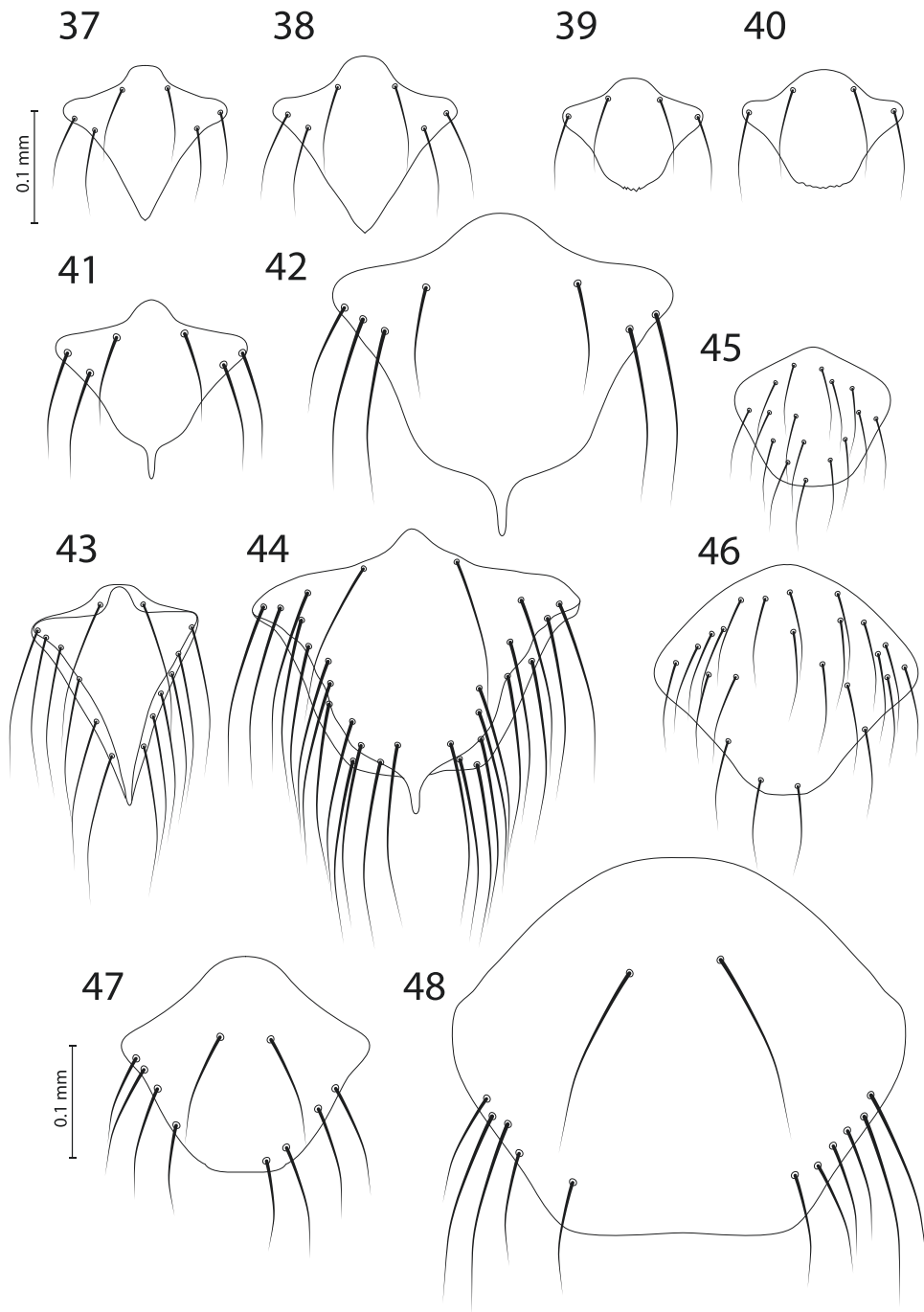
Figs. 37–48. Metasternal plate. 37 and 38, M. sylviae : 37, Male; 38, Female. 39 and 40, M. johnsoni : 39, male; 40, female. 41 and 42, M. hihii : 41, male; 42, female. 43 and 44, M. interrupta : 43, male; 44, female. 45 and 46, M. pilosa : 45, male; 46, Female. 47 and 48, M. bedfordi : 47, Male; 48, Female. All figures are drawn to the same scale.
