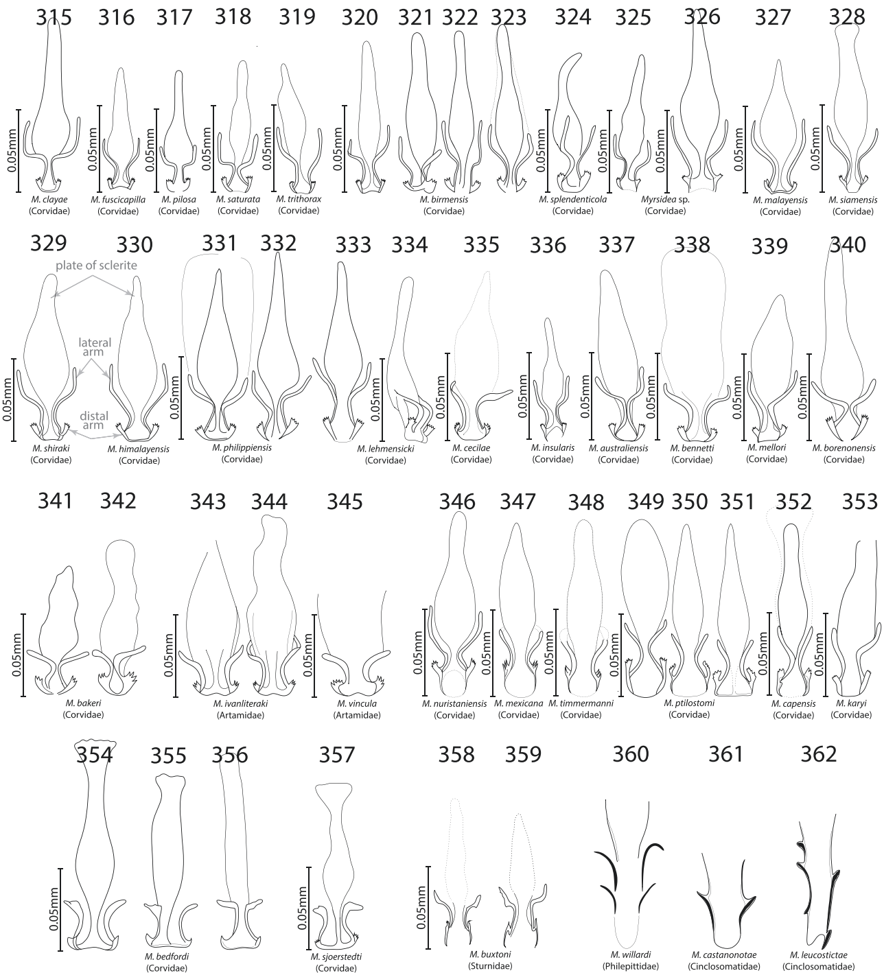
Figs. 315–362. Male genital sac sclerites. 315, M. clayae . 316, M. fuscicapilla . 317, M. pilosa . 318, M. saturata . 319, M. trithorax . 320–323, M. birmensis . 324, M. splendenticola . 325, Myrsidea sp. from Corvus typicus . 326, Myrsidea sp. from Corvus meeki . 327, M. malayensis . 328, M. siamensis . 329, M. shiraki . 330, M. himalayensis . 331–332, M. philippinensis . 333 and 334, M. lehmsicki . 335, M. ceciliae . 336, M. insularis . 337, M. australiensis . 338, M. bennetti . 339, M. mellori . 340, M. borneonensis . 341 and 342, M. bakeri . 343 and 344, M. ivanliraki . 345, M. vincula . 346, M. nuristaniensis . 347, M. mexicana . 348, M. timmermanni . 349–351, M. ptilotomi . 352, M. capensis . 353, M. karyi . 354–356, M. bedfordi . 357, M. sjoerstedti . 358 and 359, M. buxtoni . 360, M. willardi . 361, M. castanonotae . 362, M. leucostictae . Except for figures redrawn from other publications, all figures are drawn to the same scale. Scale is shown for redrawn figures if it was present in the original publications. The following figures were redrawn from the following publications: Fig. 333 from Klockenhoff (1971b); Fig. 349 from Klockenhoff (1981a); Fig. 353 from Klockenhoff (1980a) Fig. 360 from Price and Johnson (2006b); Figs. 361 and 362 from Hellenenthal and Price (2005).
