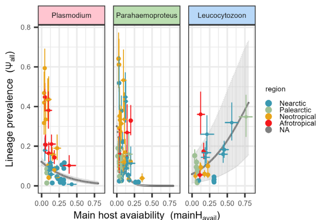
FIGURE 3 | Relationship between the estimated lineage prevalence within all locally recorded host species and main host availability (mainH.avail) for the three different haemosporidian genera Plasmodium , Parahaemoproteus and Leucocytozoon . Coloured points are posterior estimates and error bars are 95% CIs, coloured according to the four zoogeographical regions in which data were collected. Grey points and lines are the derived posterior predictions from the effect of main host availability on lineage prevalence within the model framework of the study.
